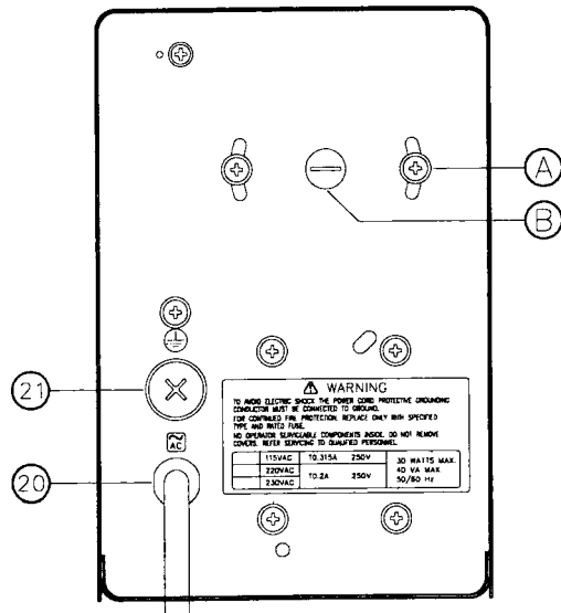
Fig. 2. Rear Panel
