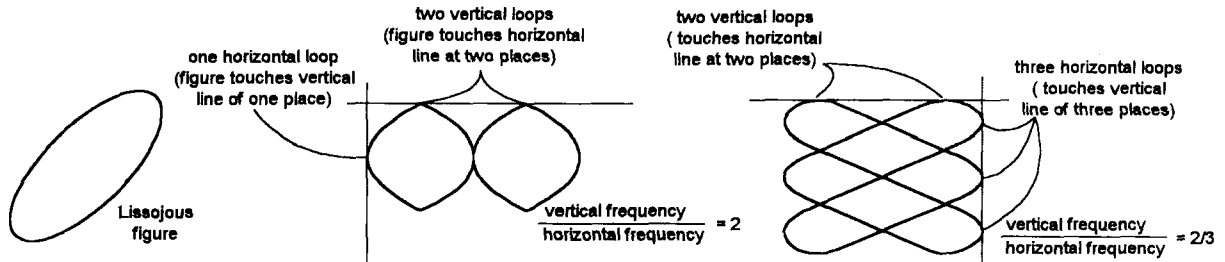
(a) Lissajous figure with vertical and horizontal inputs at the same frequency (out of phase)
